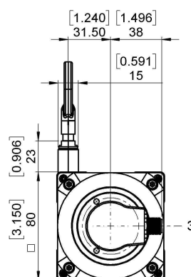
CONNECTION ORIENTATION
