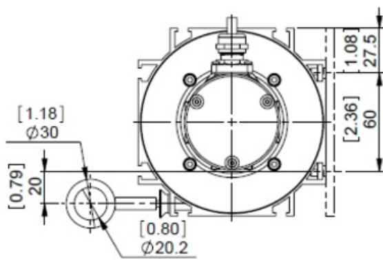
ASSEMBLING AID
