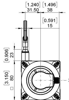
CONNECTION ORIENTATION
