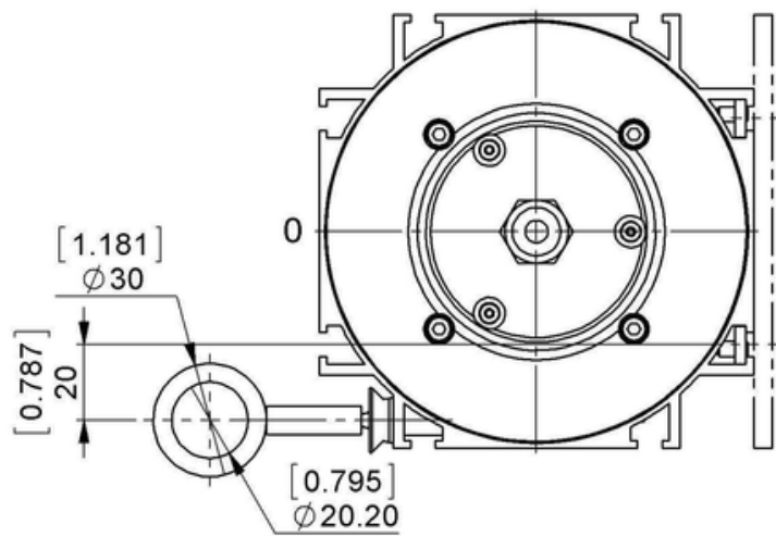
ASSEMBLING AID
