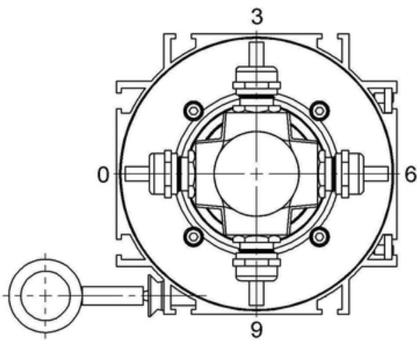
CONNECTION ORIENTATION
