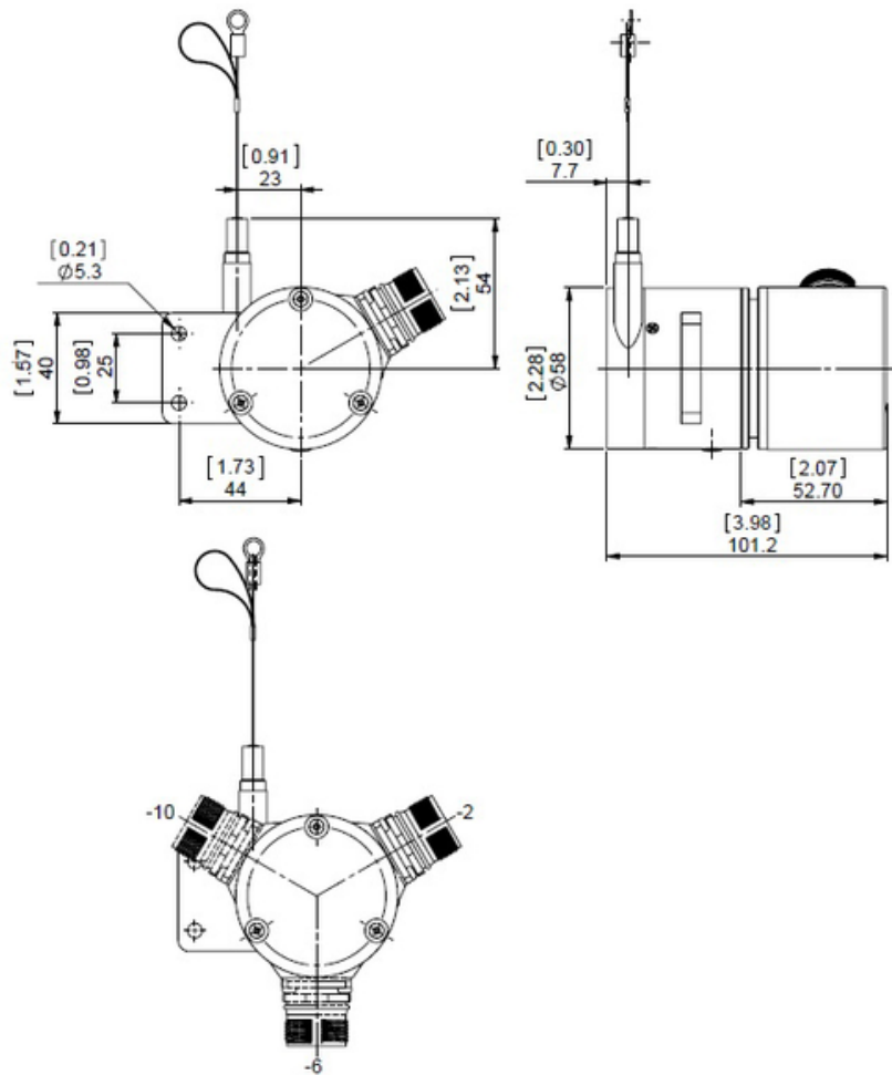
CONNECTION ORIENTATION
