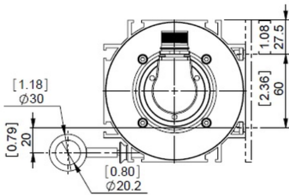
ASSEMBLING AID
