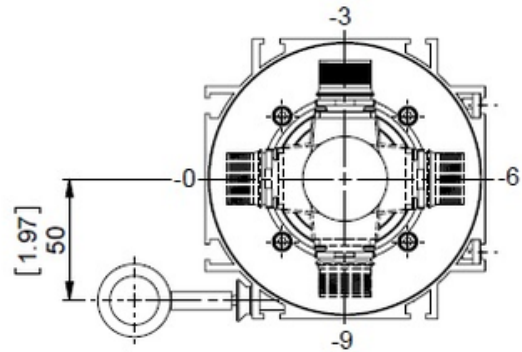
CONNECTION ORIENTATION
