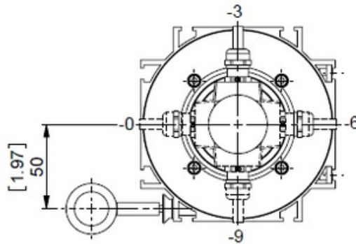
CONNECTION ORIENTATION
