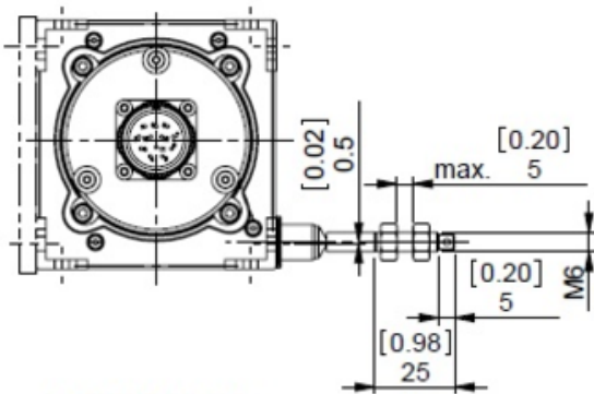
ASSEMBLING AID
