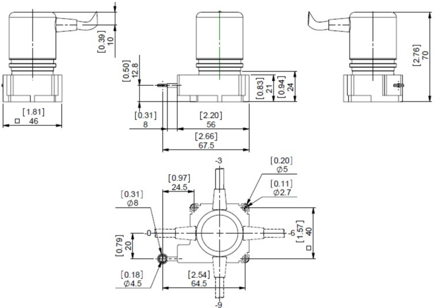
CONNECTION ORIENTATION
