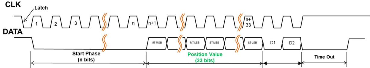
Figure 3: Protocol structure S303B
