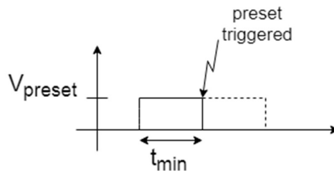
Figure 5: Preset hardware trigger.
