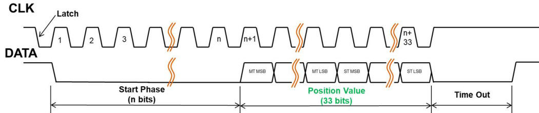
Figure 2: Protocol structure S10xB
