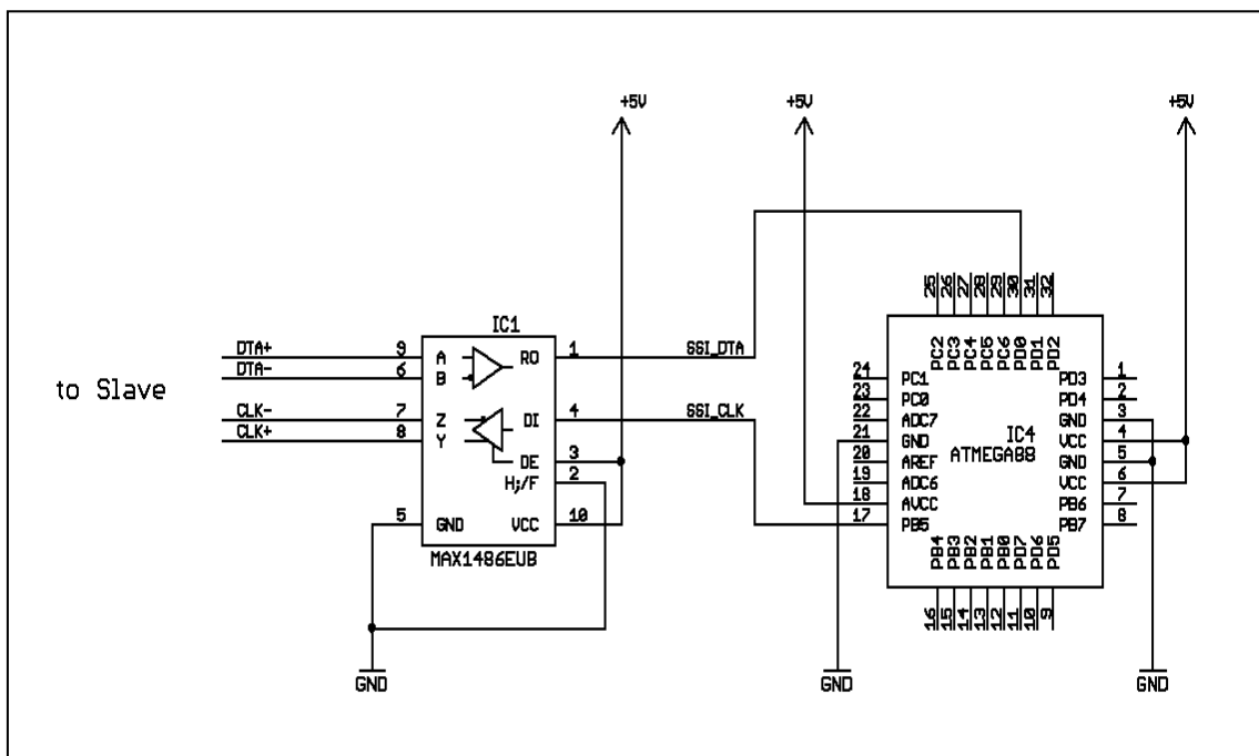
Figure 2.1: Simple SSI Master
