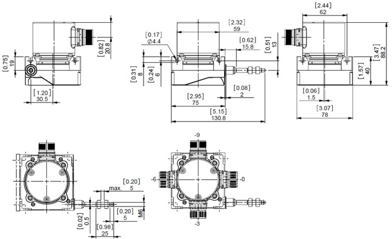
ASSEMBLING AID
