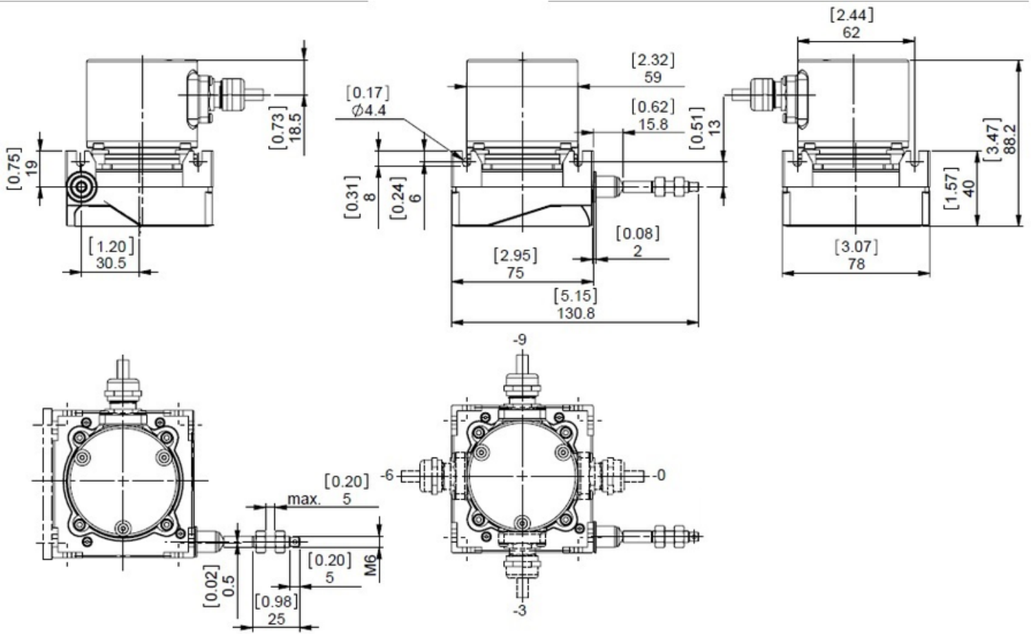
ASSEMBLING AID
