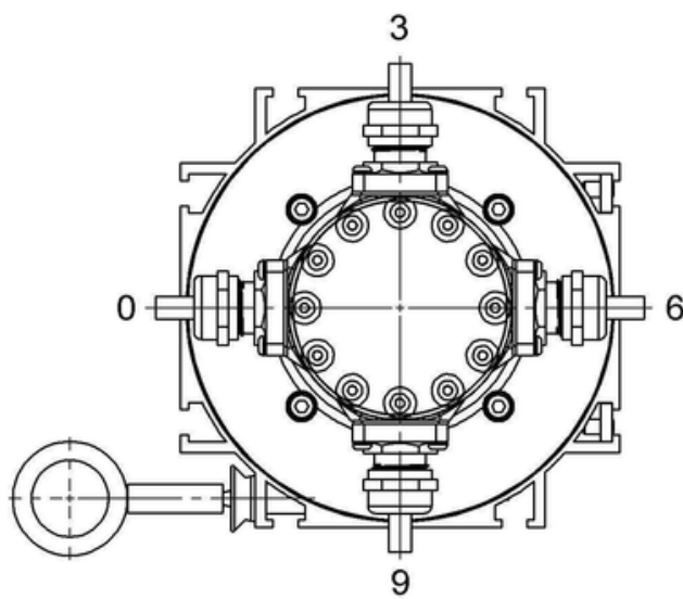
CONNECTION ORIENTATION
