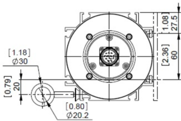
ASSEMBLING AID
