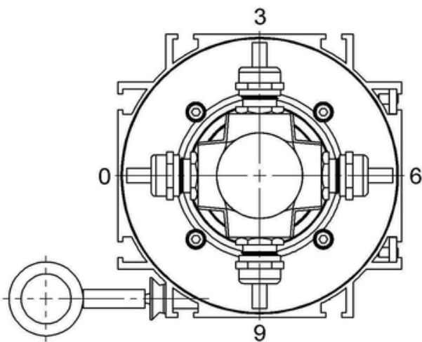
CONNECTION ORIENTATION
