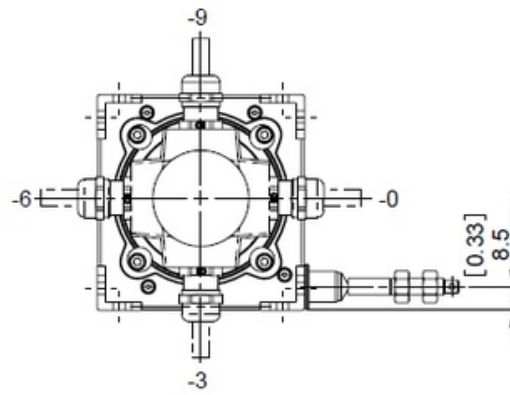
CONNECTION ORIENTATION
