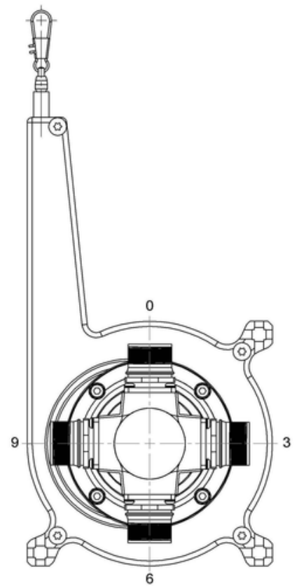
CONNECTION ORIENTATION
