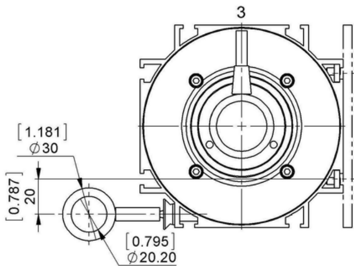
ASSEMBLING AID
