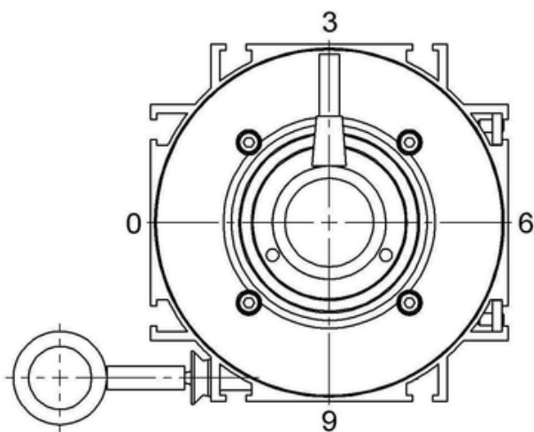
CONNECTION ORIENTATION
