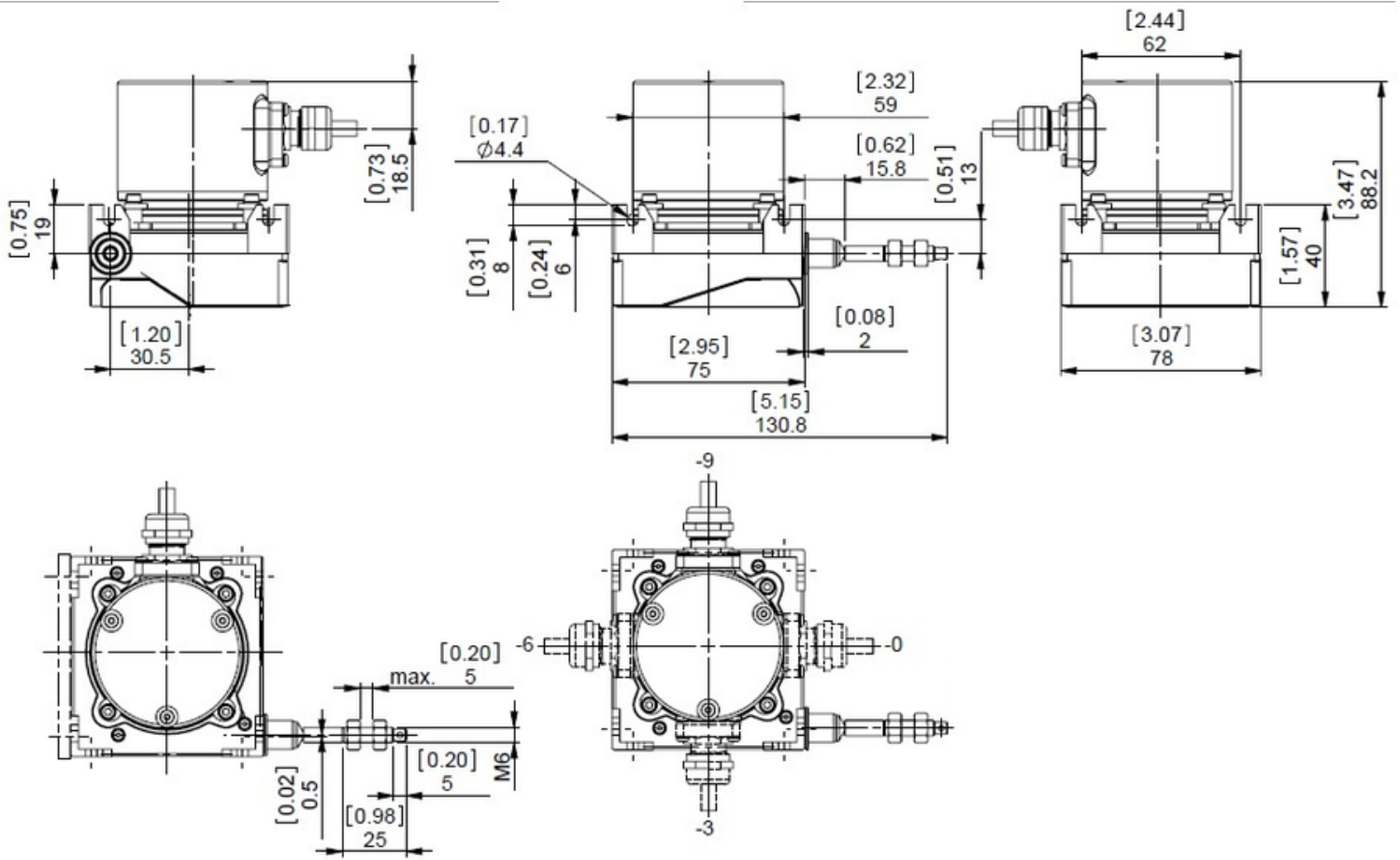
ASSEMBLING AID
