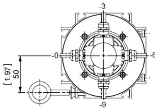
CONNECTION ORIENTATION
