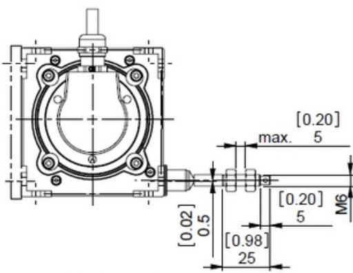
ASSEMBLING AID
