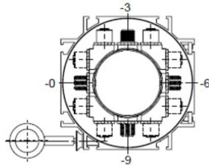
CONNECTION ORIENTATION
