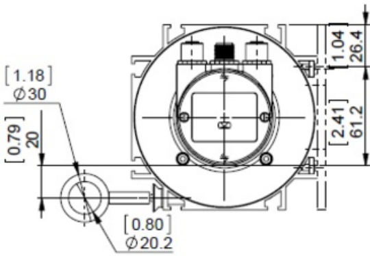
ASSEMBLING AID
