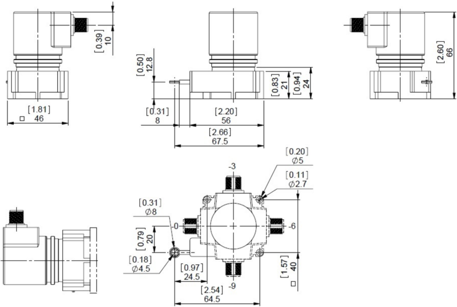
ASSEMBLING AID & CONNECTION ORIENTATION
